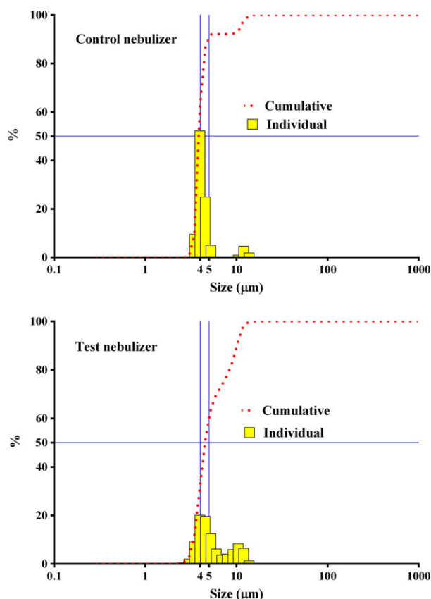
Fig. 3. Distribution of aerosol ipratropium bromide particle sizes for control (upper) and test (lower) nebulizers.
